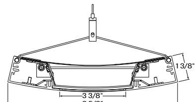
SMIPSIB - sliding cable suspension
